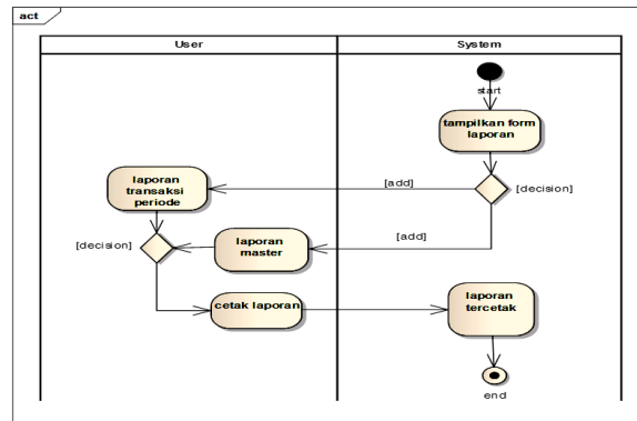
Gambar 7 Activity Diagram Mencetak Laporan
