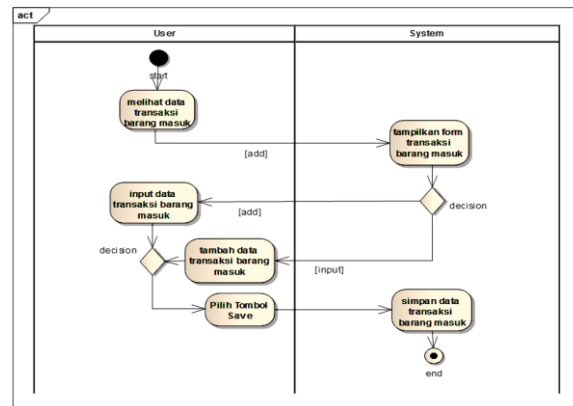
Gambar 5 Activity Diagram Transaksi Barang Masuk
